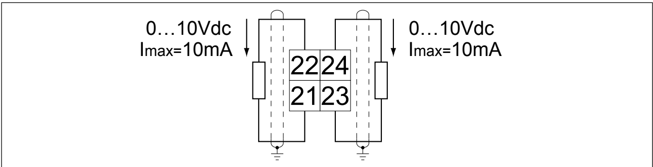
Figure 11: Connection of the analog outputs
