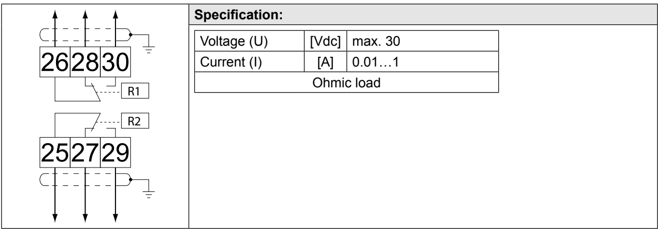
Figure 12: Connection of the relay outputs
