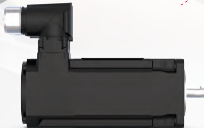
MOTOR: TA servo motor, from 0.5 - 90 Nm with a high variety of options (brake, encoder ...)
