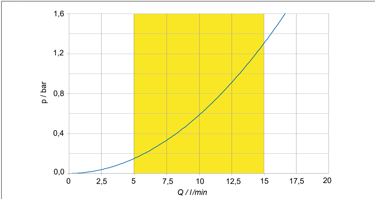
Legend Working area Figure 40: Typical pressure drop depending on the volume flow
