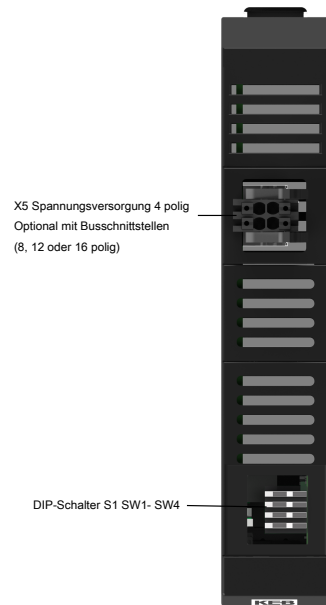
Abb. 6: C6 COMPACT 3 oben Modell 4
