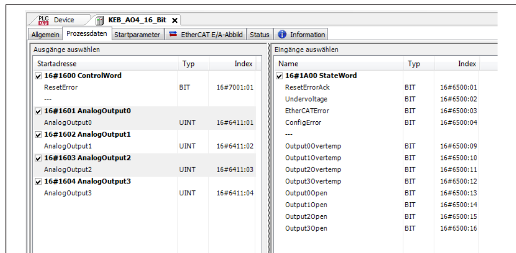
Figure 23: Process data objects
