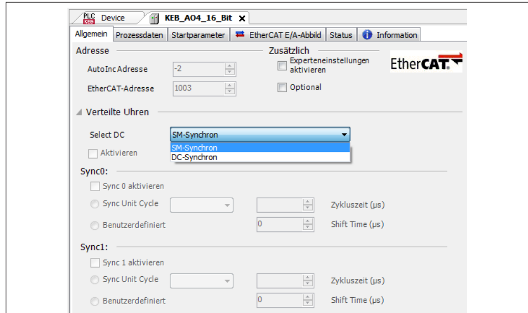
Figure 22: DC-synchron (Distributed Clocks) / SM-synchron (Sync Manager)
