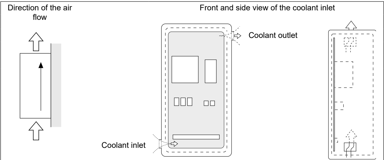
Figure 5: Control cabinet ventilation
